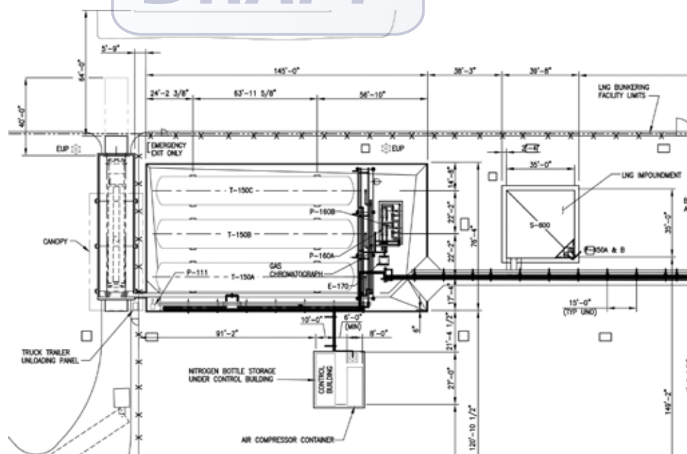
Figure 4. The plot plan: LNG bunkering facility.
